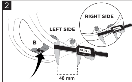
B - (1 PCS)
